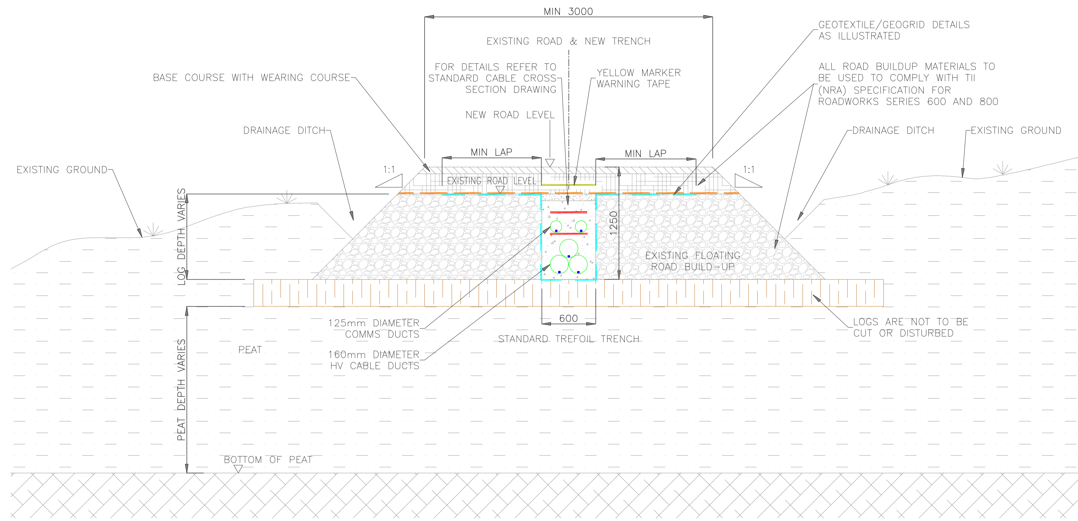
SECTION THROUGH UPGRADED FLOATING ROAD PEAT DEPTH >2.5m
